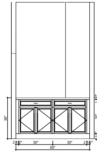
6-D Elevation(1/4"=1'-0")
