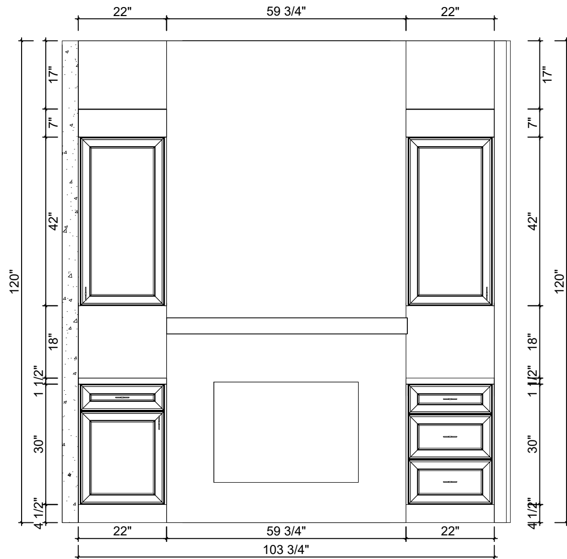
1-B Elevation(1/2"=1'-0")
