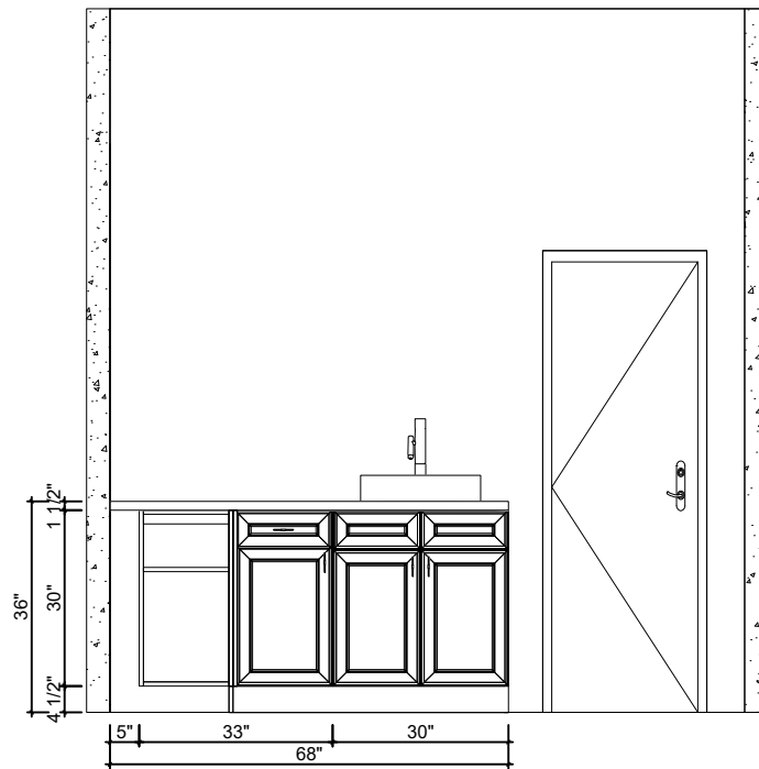
2-D Elevation(1/3"=1'-0")
