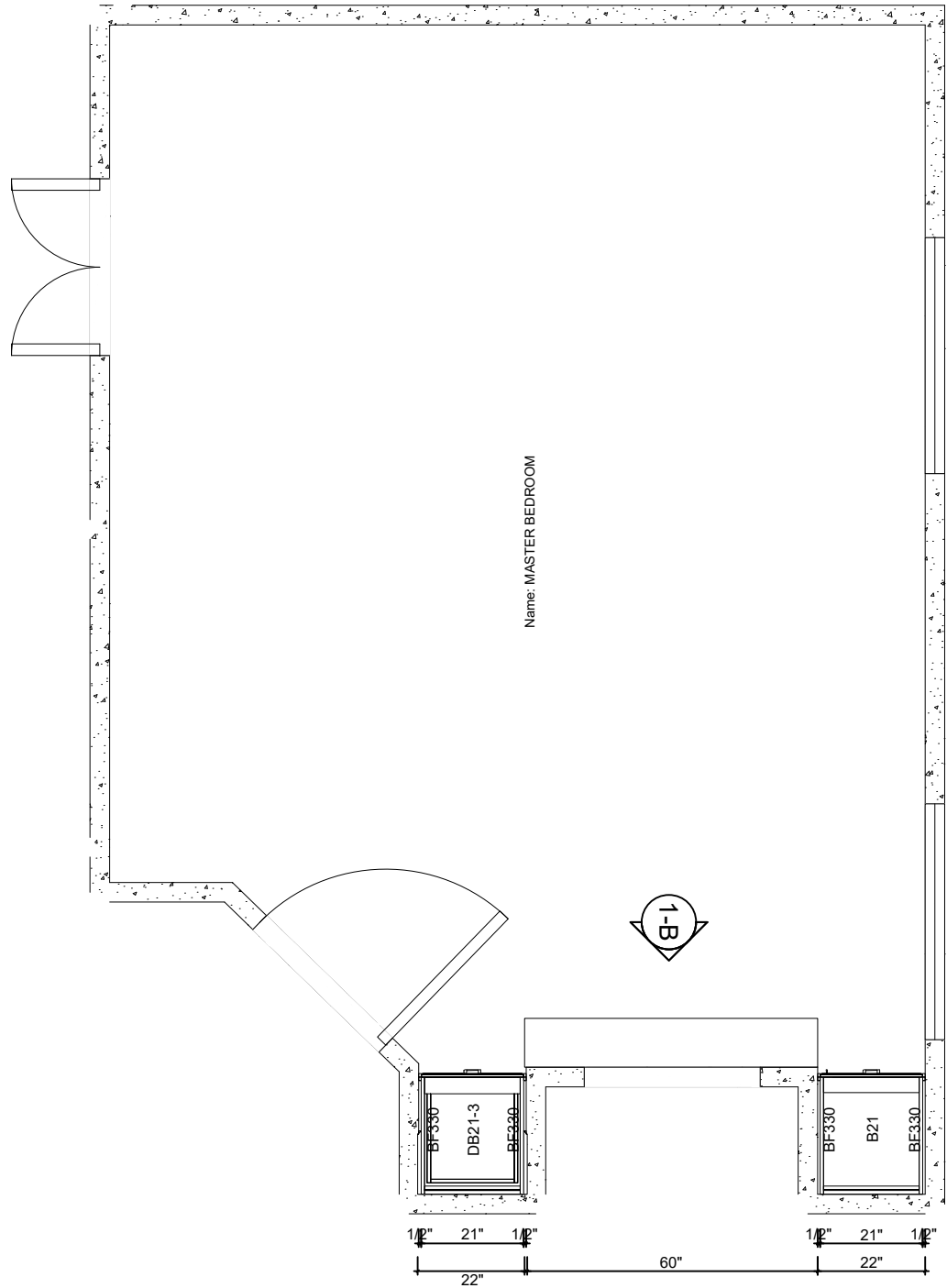
Base Unit Plan View(1/3"=1'-0")
