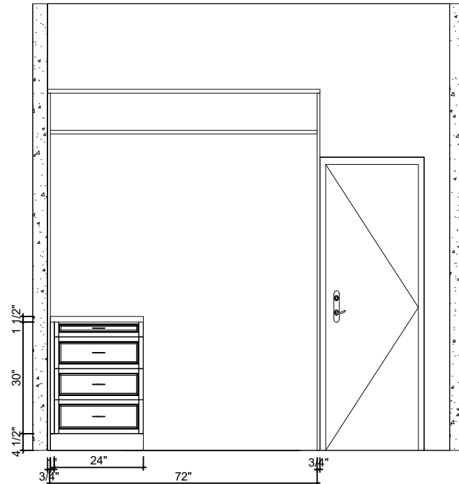
1-B Elevation(1/3"=1'-0")
