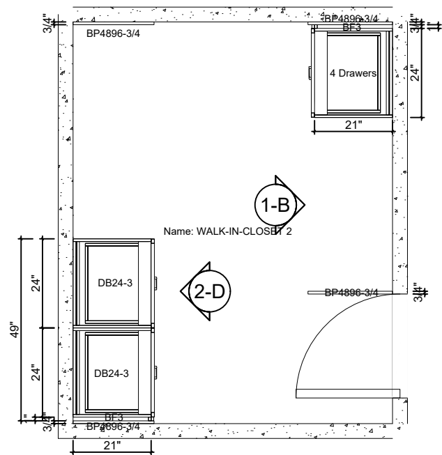
Base unit plan(1/3"=1'-0")
