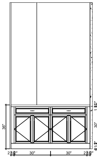
5-D Elevation(1/4"=1'-0")
