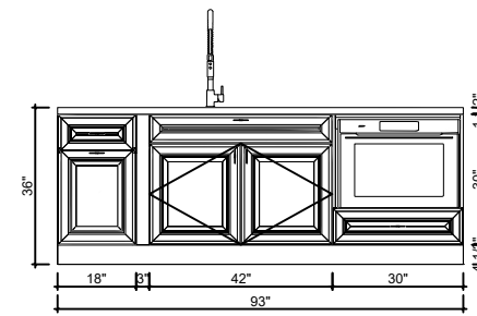
4-D Elevation(1/4"=1'-0")
