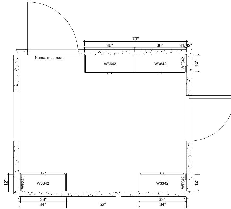
Wall unit plan(1/3"=1'-0")
