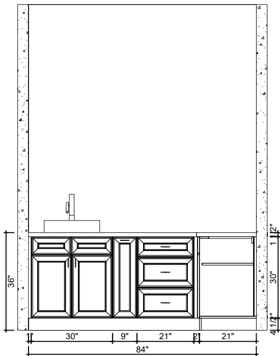
1-C Elevation(1/3"=1'-0")
