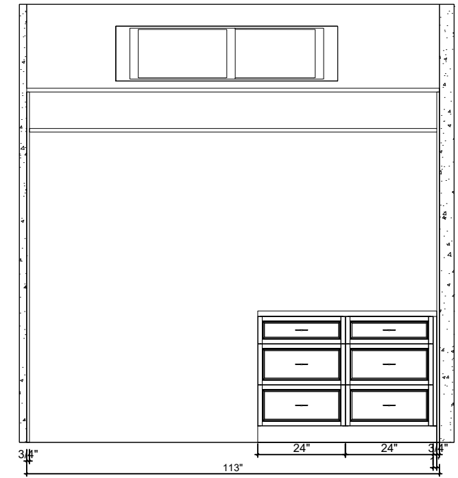
2-D Elevation(1/3"=1'-0")
