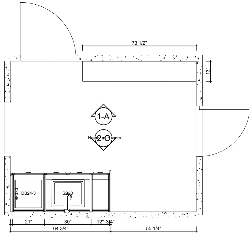
Base unit plan(1/3"=1'-0")
