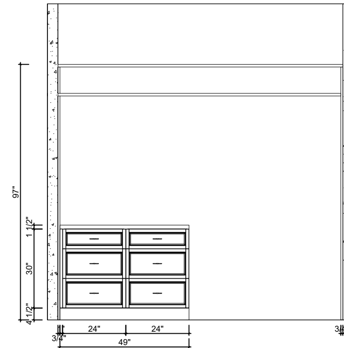
2-D Elevation(1/3"=1'-0")
