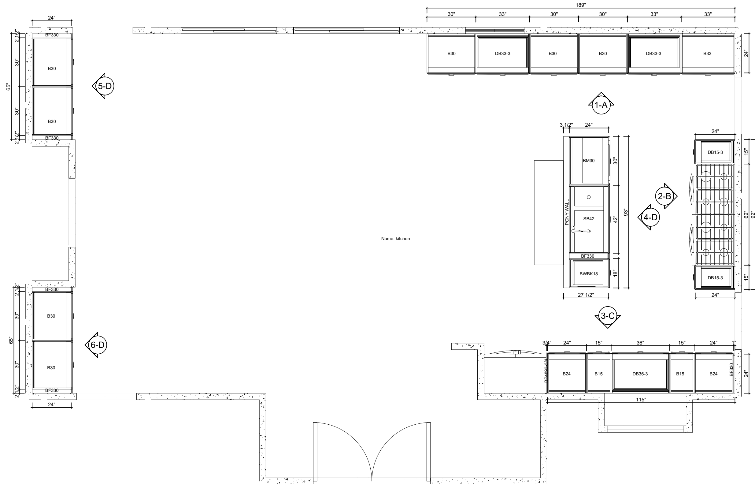
Base Unit Plan View(1/3"=1'-0")
