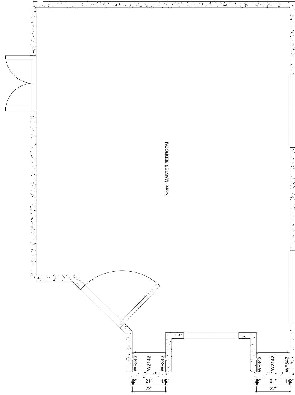
Wall Unit Plan View(1/3"=1'-0")
