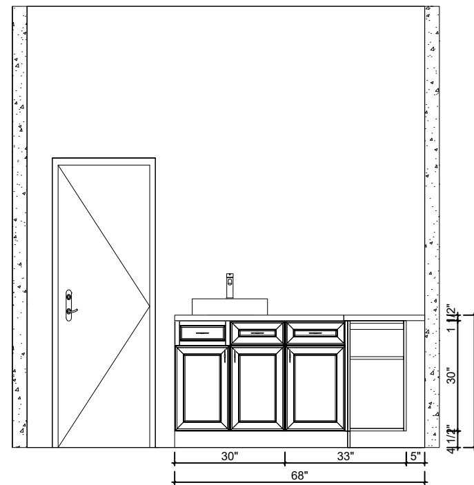
2-D Elevation(1/3"=1'-0")
