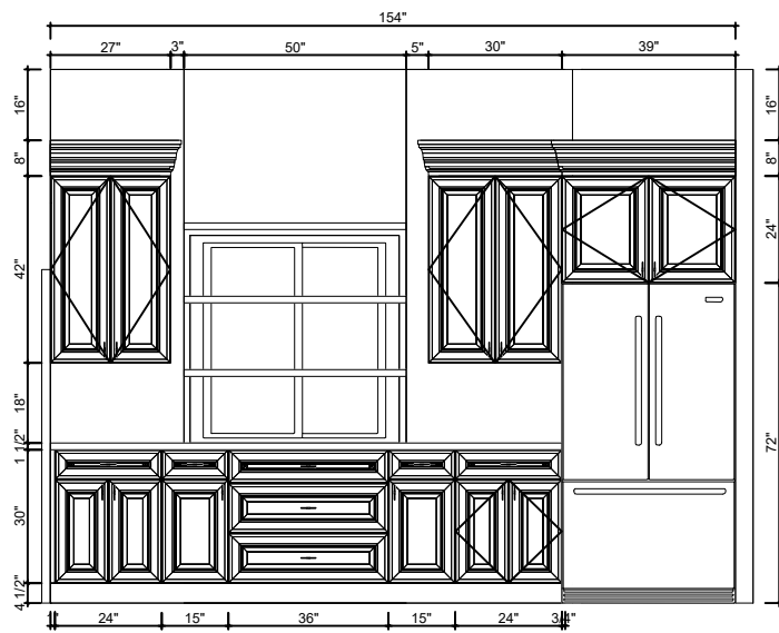
3-C Elevation(1/4"=1'-0")
