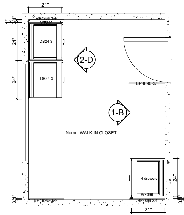
Base unit plan(1/3"=1'-0")
