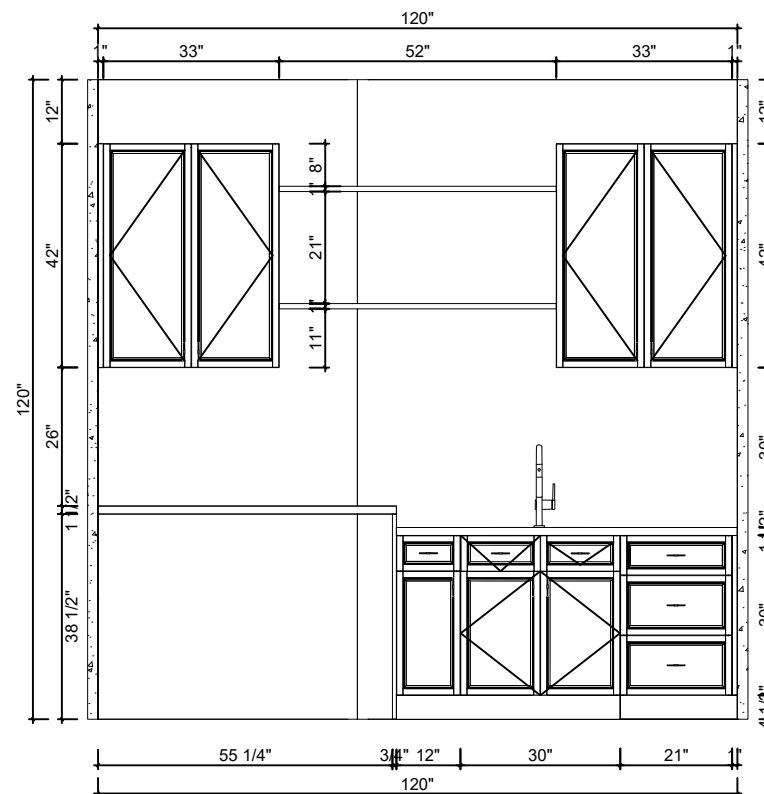
2-C Elevation(1/3"=1'-0")
