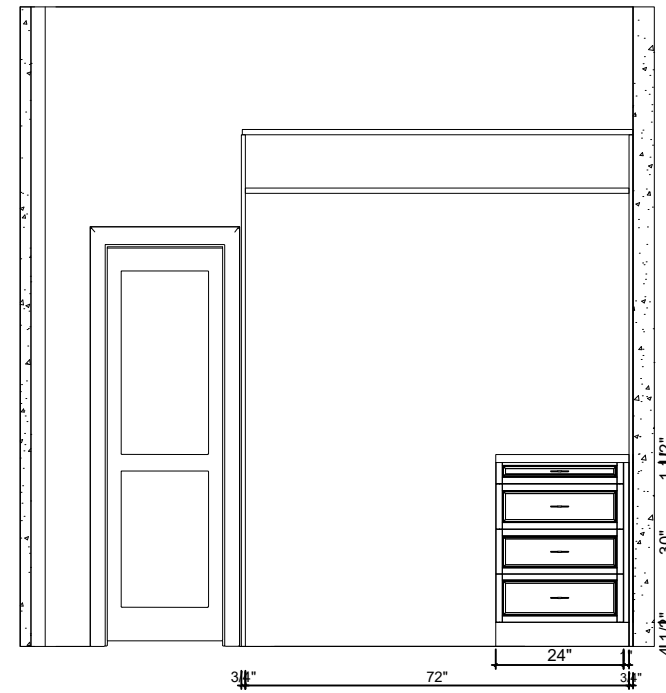
1-B Elevation(1/3"=1'-0")
