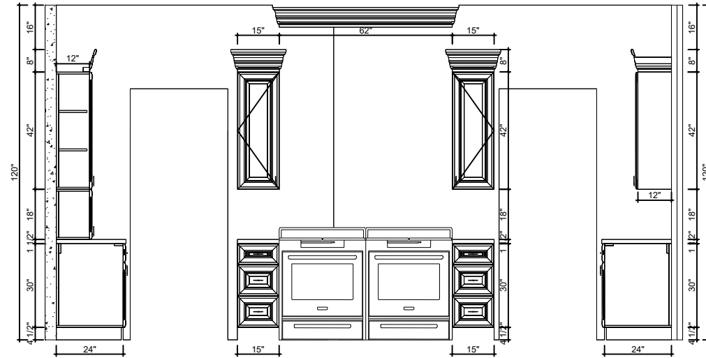
2-B Elevation(1/4"=1'-0")
