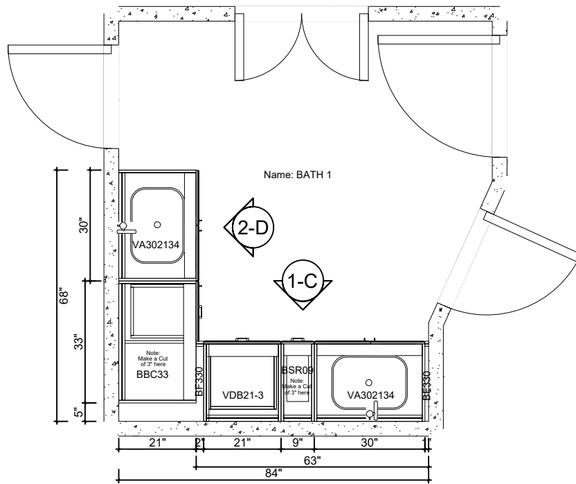
Base Unit Plan View(1/3"=1'-0")
