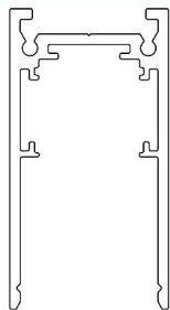
Ceiling type, using screws to fix the track on the ceiling
