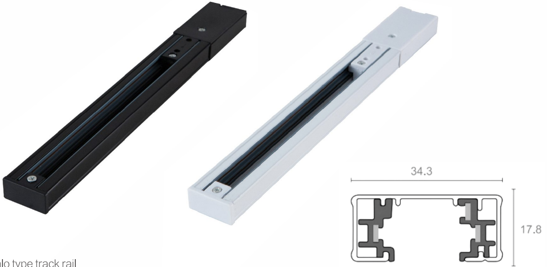
Halo type track rail Length: 2ft, 4ft, 6ft, 8ft Surface mounted or suspension type
