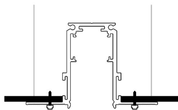
Place the track into the slot and lock the track to the ceiling with M4 tapping screws
