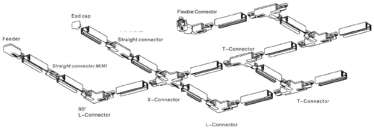
Installation diagram
