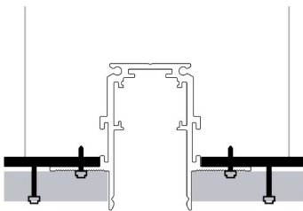
Install the gypsum board on the track and block the wings of the track
