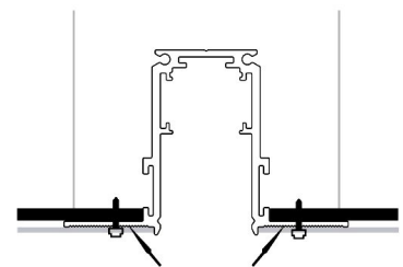
Batch the track surface with ash, covering the exposed wing as shown
