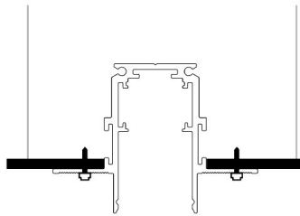
Place the track into the slot and lock the track to the ceiling with M4 tapping screws
